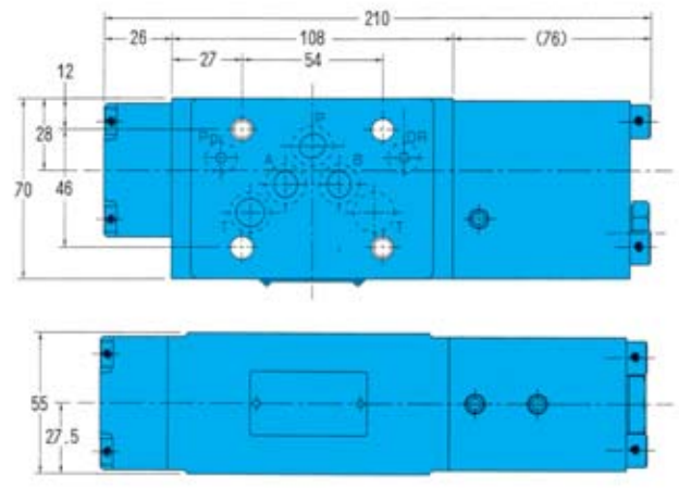
JHF-03080 (E)
