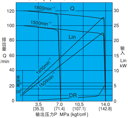
VDC-3A(B)-1A5-20
