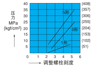
ORH-G04-P*-10
