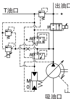
PZ-2B/3B/5B
