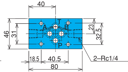
OK-G01-T-H-20
