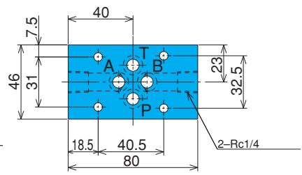
OK-G01-W-20
