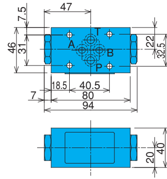
OCV-G01-W-20
