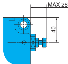
(C) FT-G03-**-F-22
