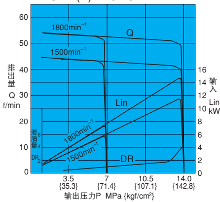
VDC-2A(B)-1A5-20
