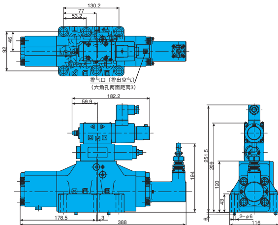
ESH-G06
