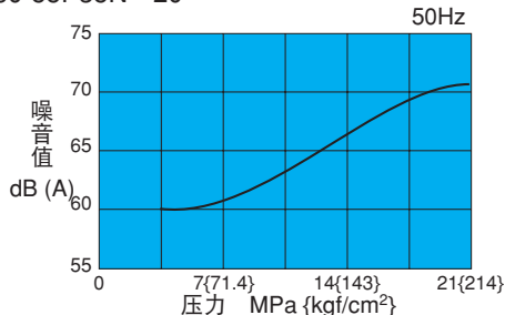
NNP-60-55P35N*-20
