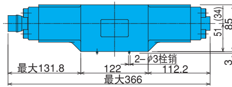
OFH-G04-A200-X/Y-10
