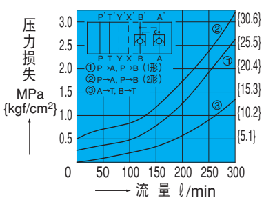
OPH-G04-W*-10
