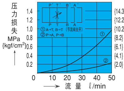
OY-G01-T-20
