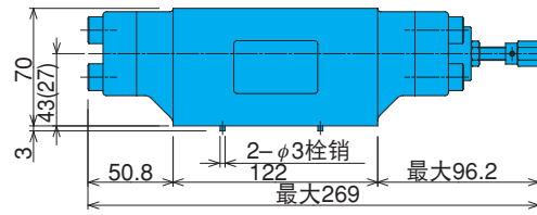
OYH-G04-B-X-10
