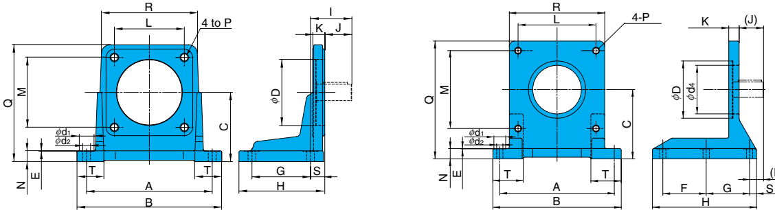
Foot Mounting Installation Measurement Chart IHM-55-10
