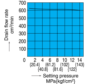
Pressure - Drain Rate Characteristics OGS-G01-P21-K-**-22
