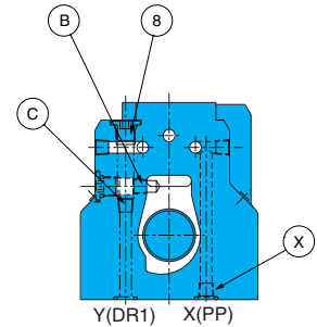
Cross-sectional R-R
