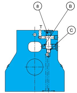
Cross-sectional R-R
