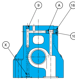
Cross-sectional P-P
